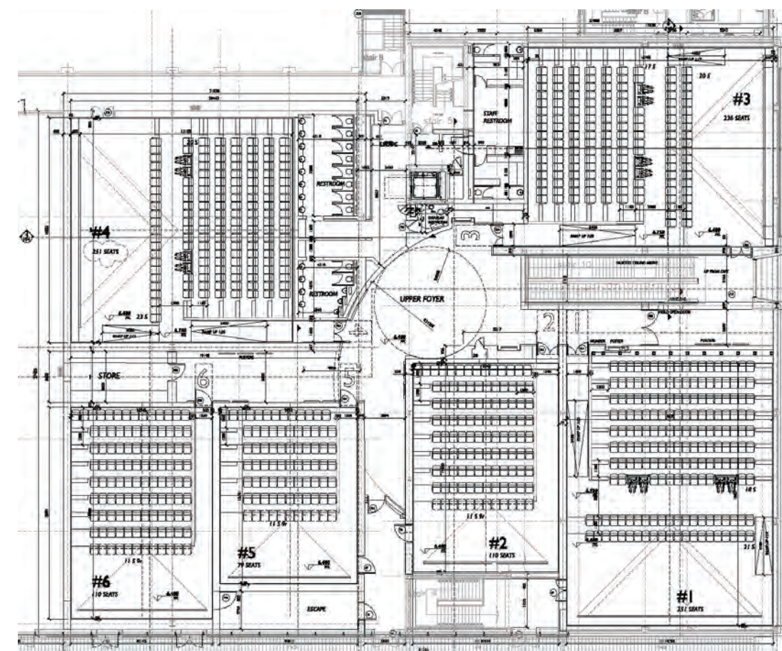
New Brighton - 1st Floor Plan
